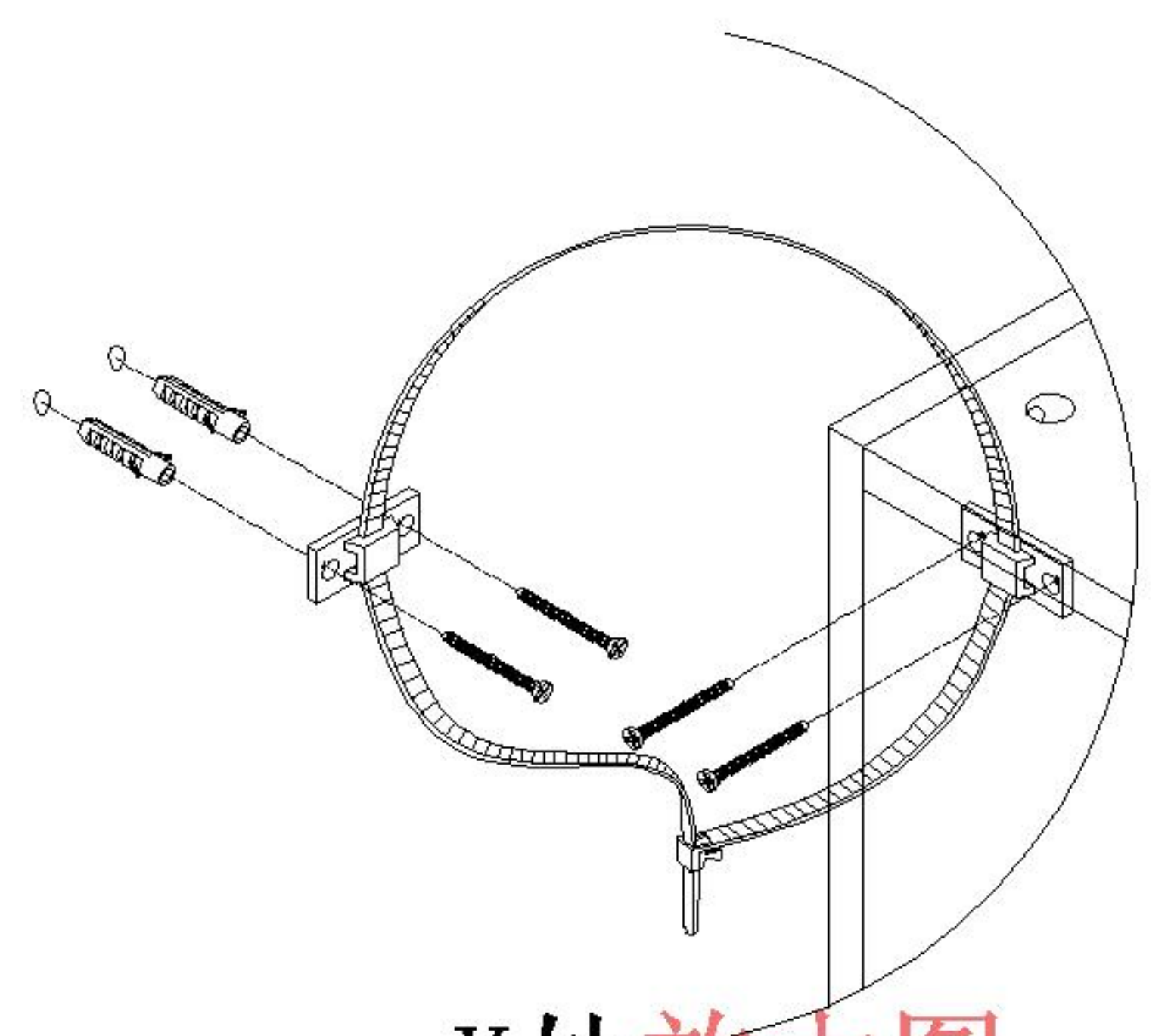
X处放大图 Enlarged view at X
