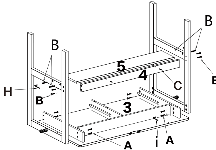
Step2:Install left and right tripod, lower brace, storage board
